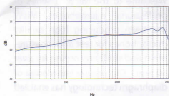
Typical Frequency Response of i266 at 20cm from the source
