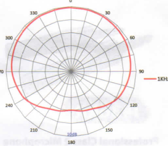
Polar Pattern for i456
